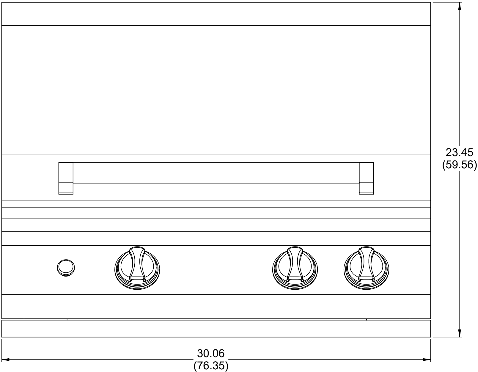
FRONT VIEW
