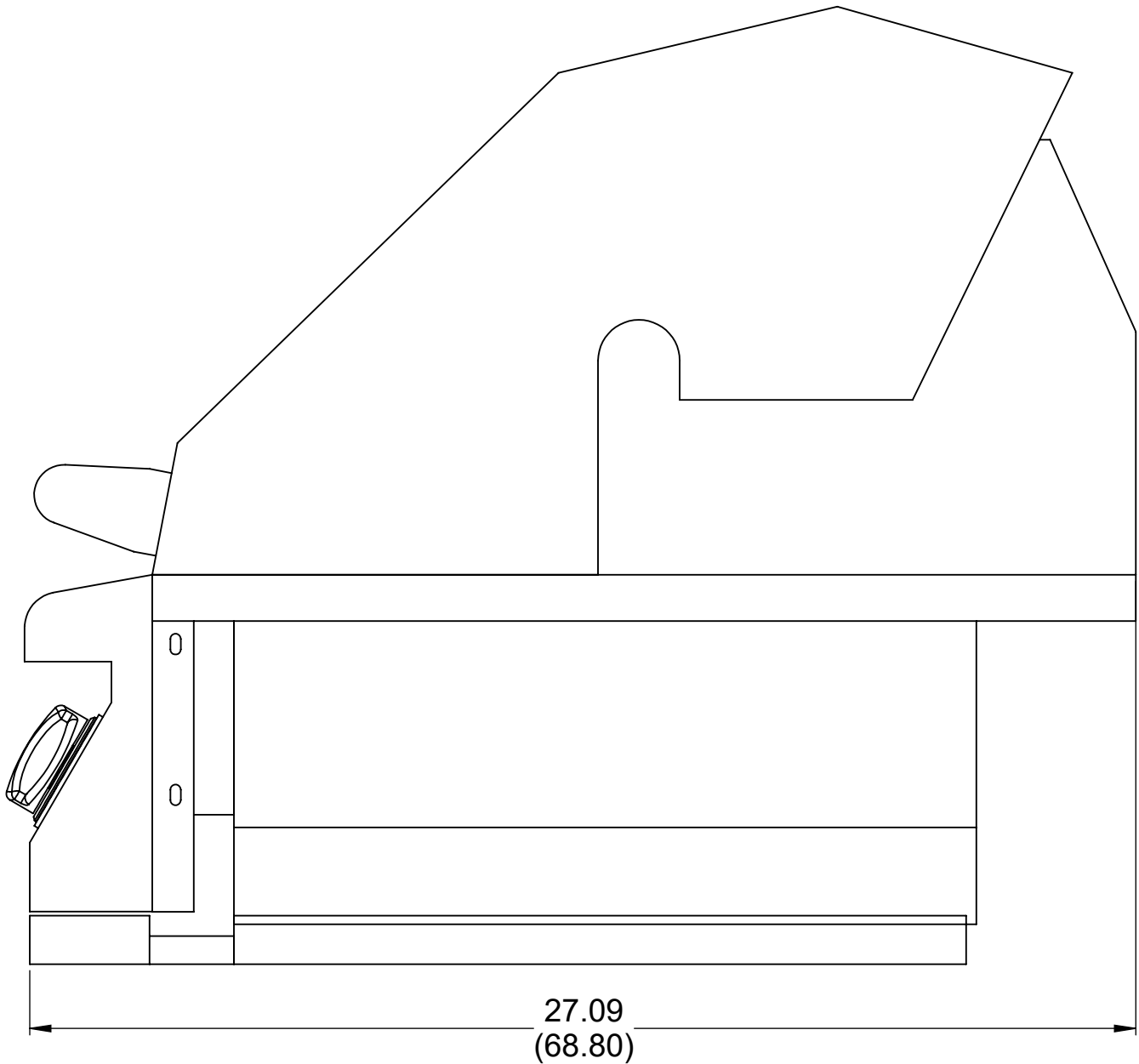
SIDE VIEW
