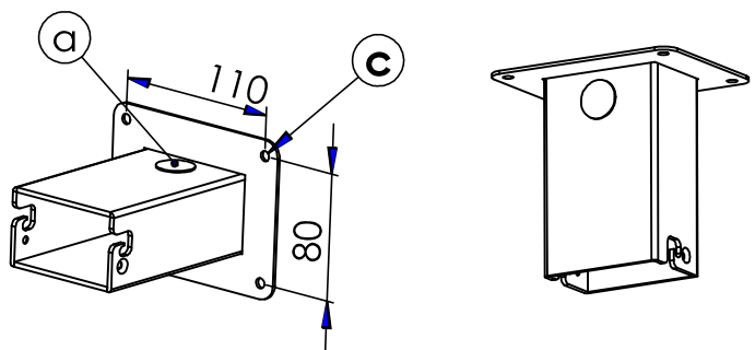
Wall mount
