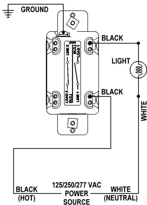
TYPICAL WIRING
